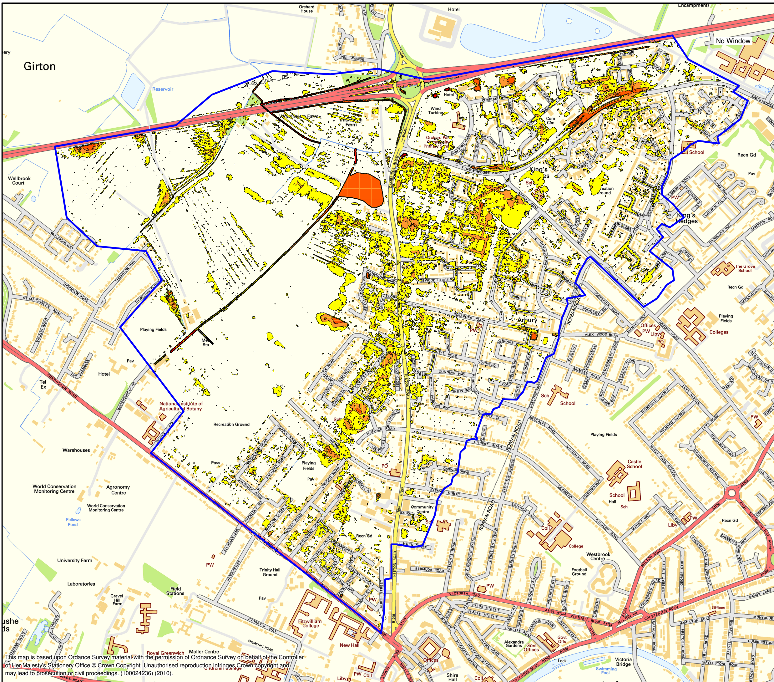
FIGURE F40 3.3% AEP "DO MINIMUM" PLUVIAL MODELLING MAXIMUM DEPTH KING'S HEDGES AND ARBURY
